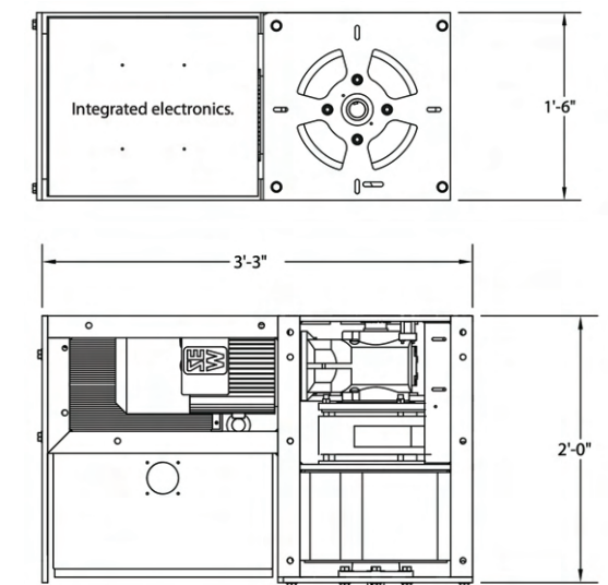
Top: Foy DW-V3 Elevation Bottom: Foy DW-V3 Section
